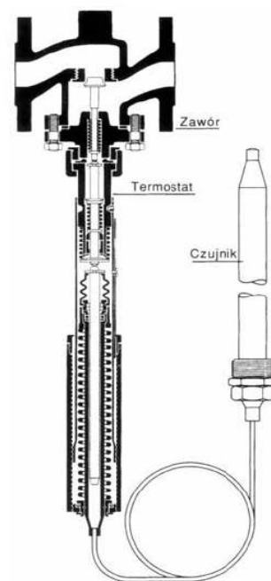
Regulator temperatury
